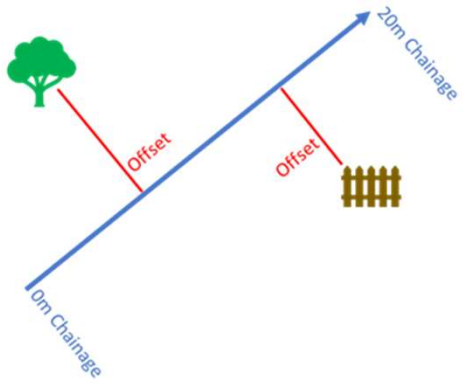
Chainage and Offset Survey
